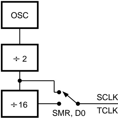
Figure 40. SCLK Circuit
