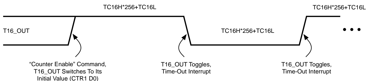
Figure 33. T16_OUT in Modulo-N Mode
