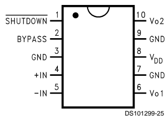
Top View Order Number LM4876MM See NS Package Number MUB10A
